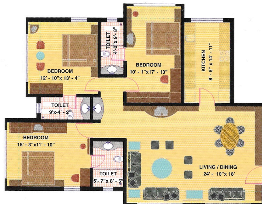
B-Wing THIRD FLOOR PLAN
