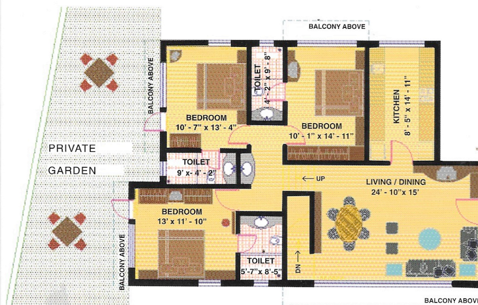
B-Wing GROUND FLOOR PLAN ( Basement below )
