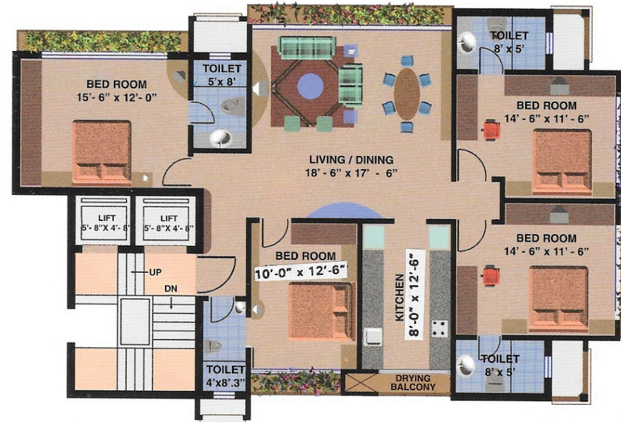
A-Wing TYPICAL FLOOR PLAN - 4 BHK
